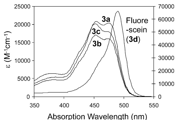
Figure 1. The molar extinction curves of the mono- O -alkylated fluorescein derivatives in comparison to fluorescein. Absorption spectra for 3'- O -butyl fluorescein 3a , 3'- O -EME fluorescein 3b , 3'- O -MEM fluorescein 3c and fluorescein were obtained at pH 7.0 (30 \mu M in 10 mM PBS). The scale on the left is for 3a–c and on the right for fluorescein ( 3d ).
