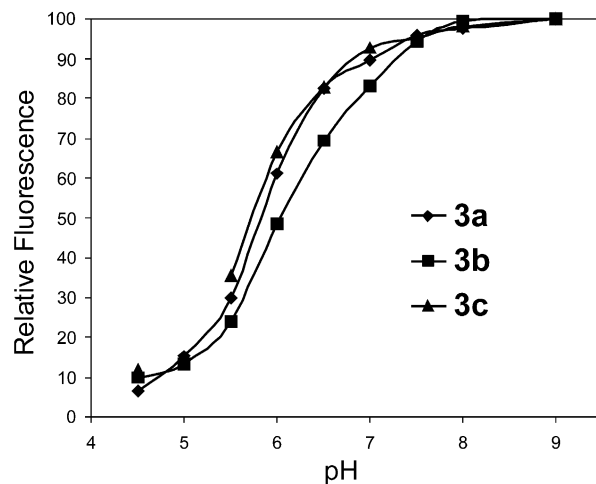
Figure 3. Relative fluorescence as a function of pH for the fluorescein derivatives. The derivatives were excited at 467 nm and detected at 518 nm in 10 mM PBS at the indicated pH and normalized to the maximum intensity for each derivative.
