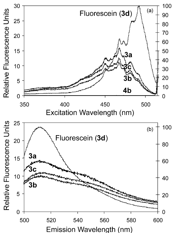
Figure 2. Fluorescence spectra of the fluorescein derivatives in comparison to fluorescein. A. Excitation spectra of 3'- O -butyl fluorescein 3a , 3'- O -EME fluorescein 3b , 3'- O -MEM fluorescein 3c and 6'- O -acetyl-3'- O -EME fluorescein 4b , (1 \mu M in 10 mM pH 7.0 PBS, detection at 518 nm) B. Emission spectra of butyl fluorescein 3a , EME fluorescein 3b , and MEM fluorescein 3c . (1 \mu M in 10 mM pH 7.0 PBS, excitation at 467 nm). The emission intensity was normalized to 100 for the maximum emission intensity of fluorescein (excitation at 492). The scale is on the left for 3a–c , and 4b , and on the right for fluorescein ( 3d ).
